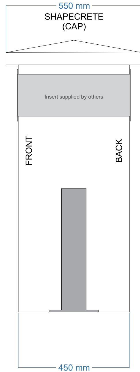
SIDE VIEW
