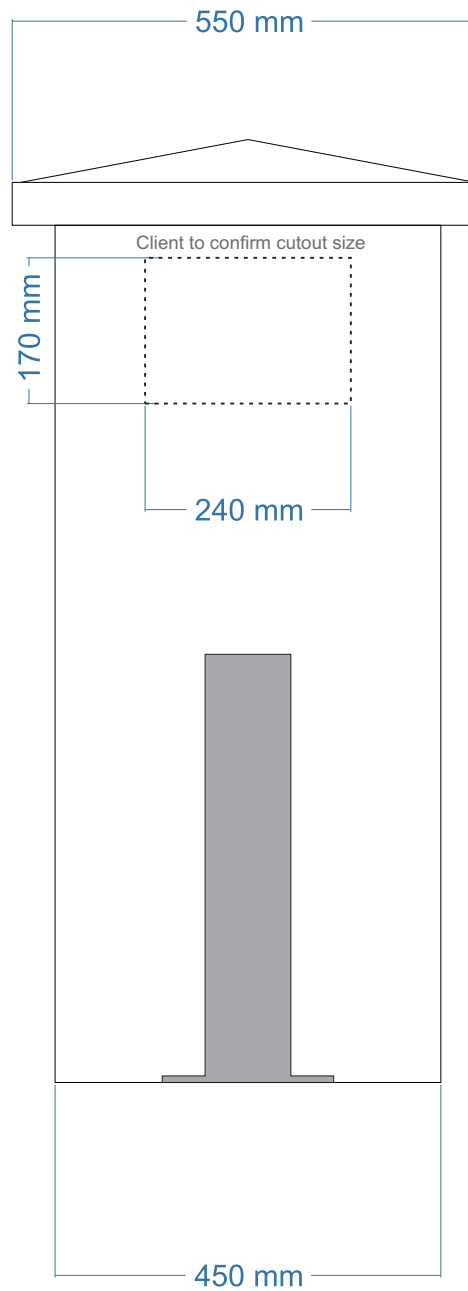
BACK VIEW
