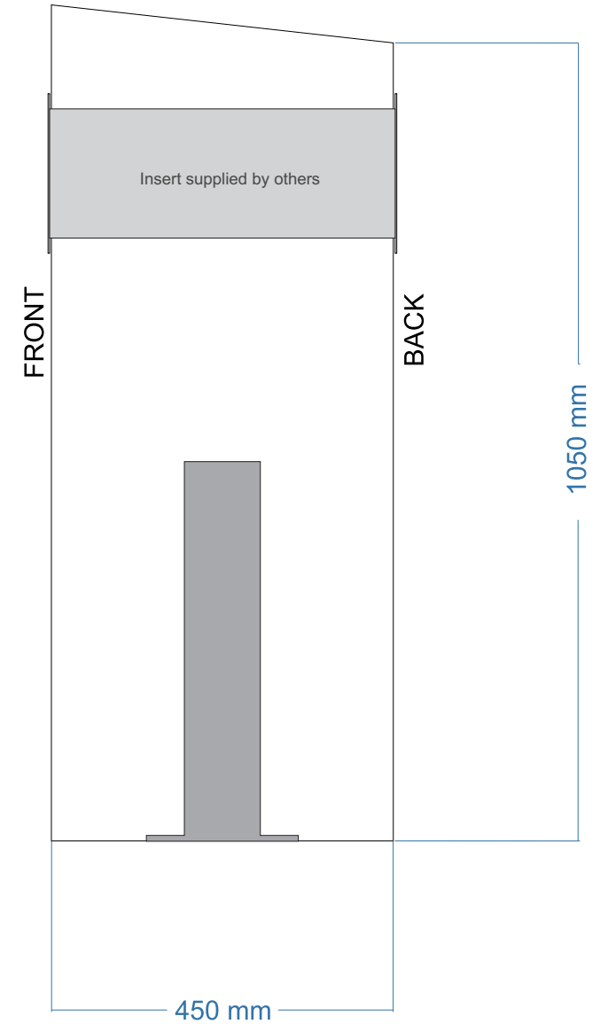
SIDE VIEW
